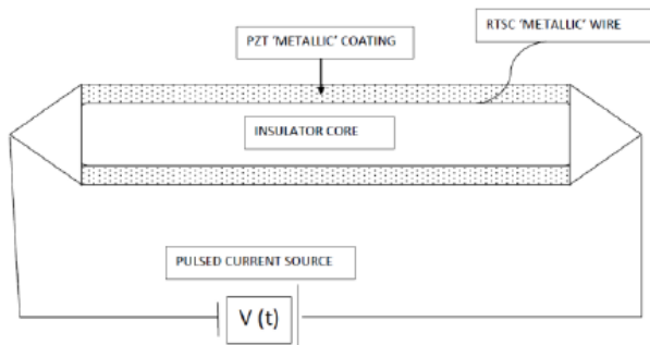
FIGURE 1 - CROSS-SECTIONAL VIEW OF RTSC WIRE
